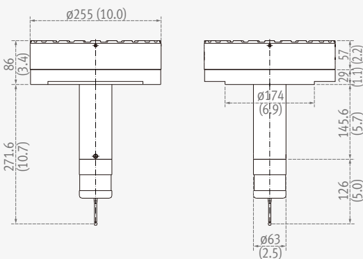
RMP60 PROBE option
