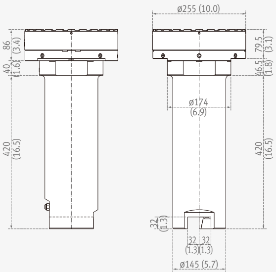
ID TOOL HOLDER option
