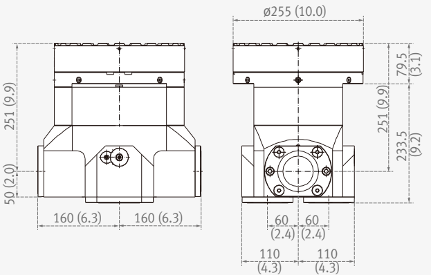
CAPTO-C8 QUAD TOOL HOLDER option
