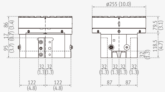
QUAD TOOL HOLDER option
