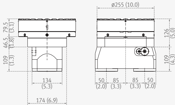
CAPTO-C8 DUAL-OD HOLDER option
