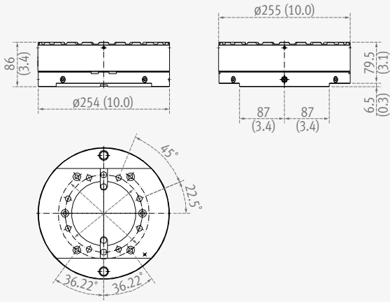
BASE TOOL HOLDER option
