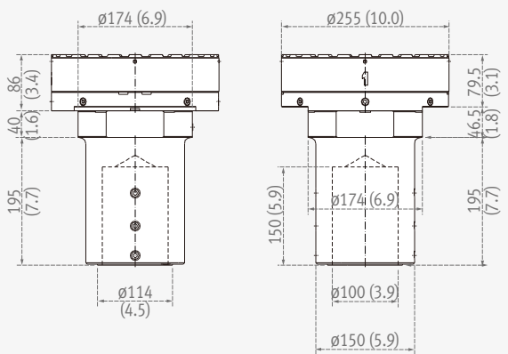
BORING TOOL HOLDER option
