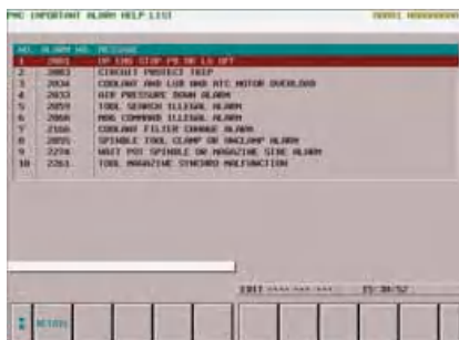
Alarm guidance Recovery method for important alarms is displayed on the screen.
